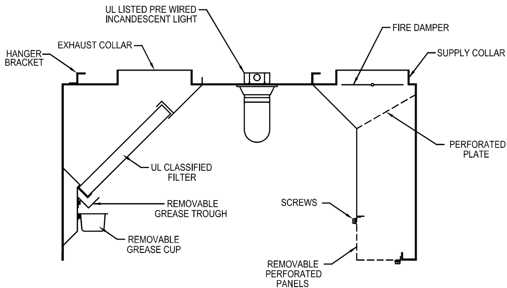
SECTION VIEW
