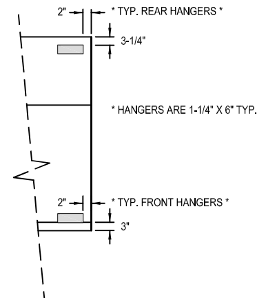
HANGER LOCATION
