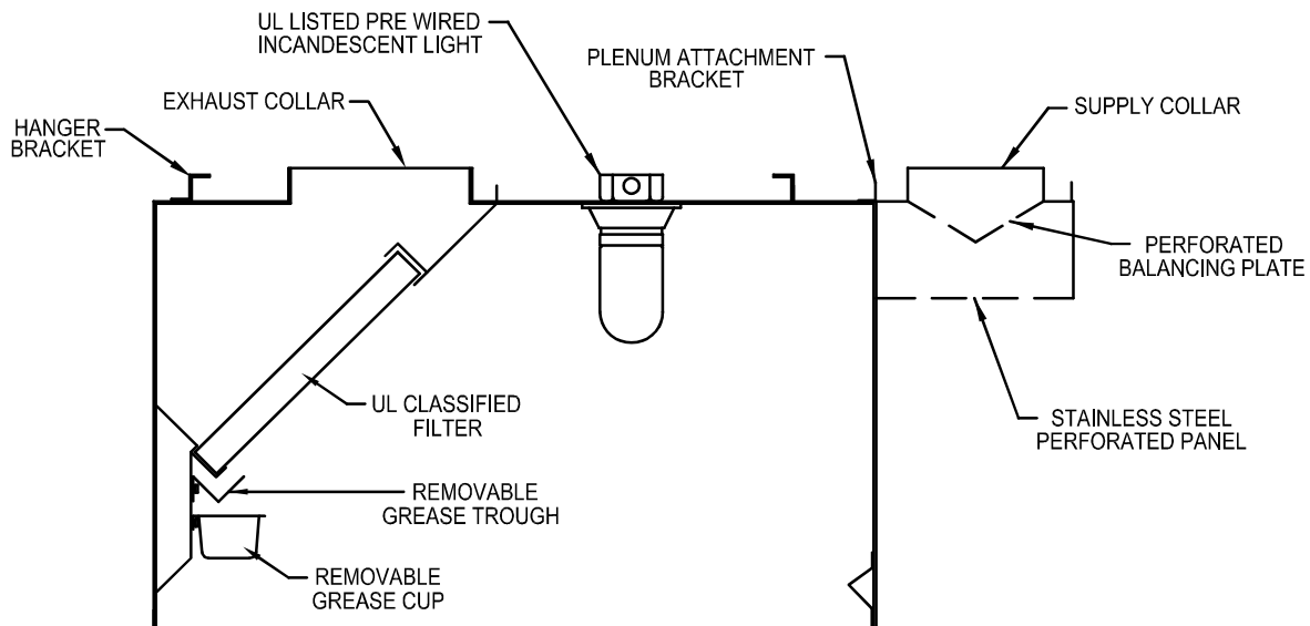
Section View
