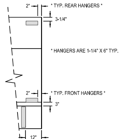
HANGER LOCATION
