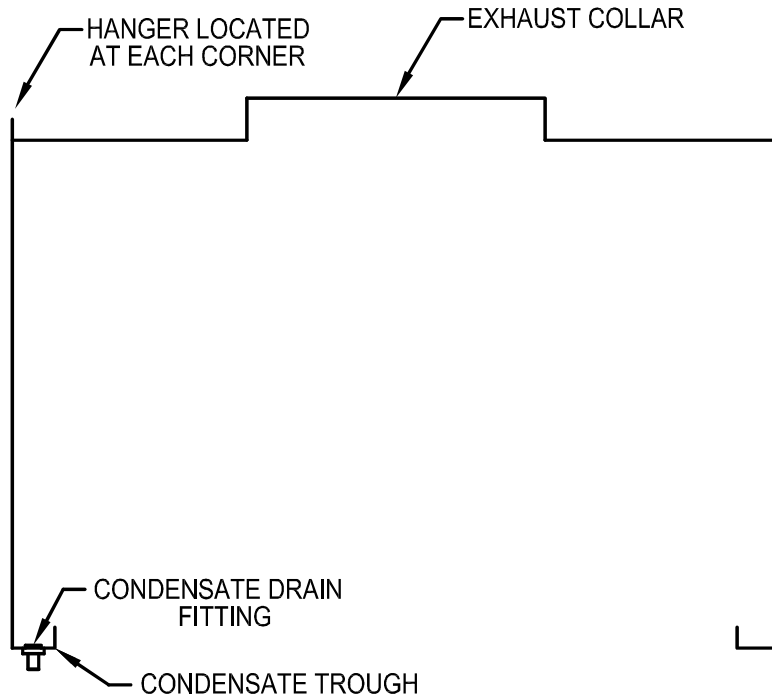
SECTION VIEW
