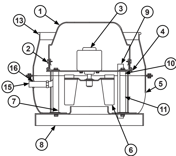
ACRU-D Sizes 70-100
