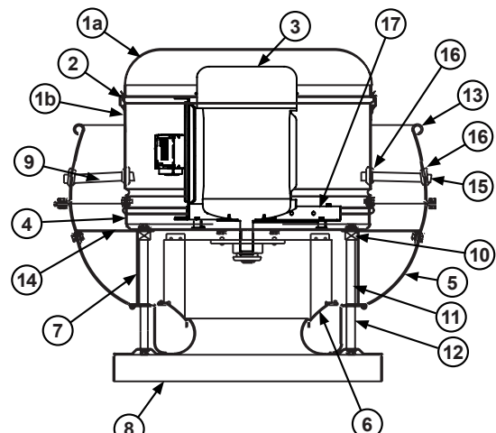
ACRU-D Sizes 150-300 Base Mount
